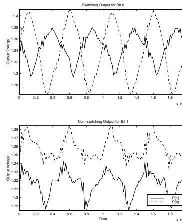
Fig. 2: Measured response of the Hamming decoder.
