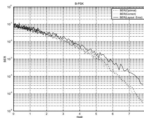
Fig. 1: Simulation results using VHDL model.
